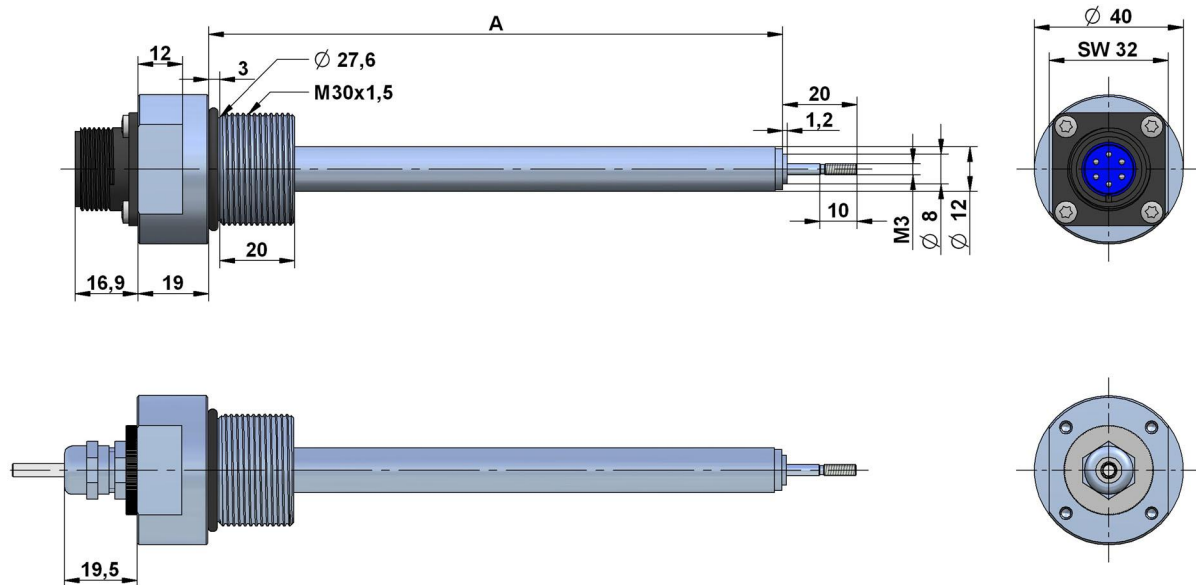
flange type with thread M30 x 1,5
