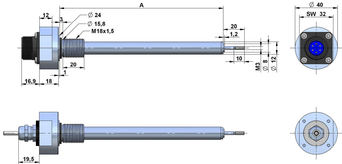
flange type with thread M18 x 1,5
